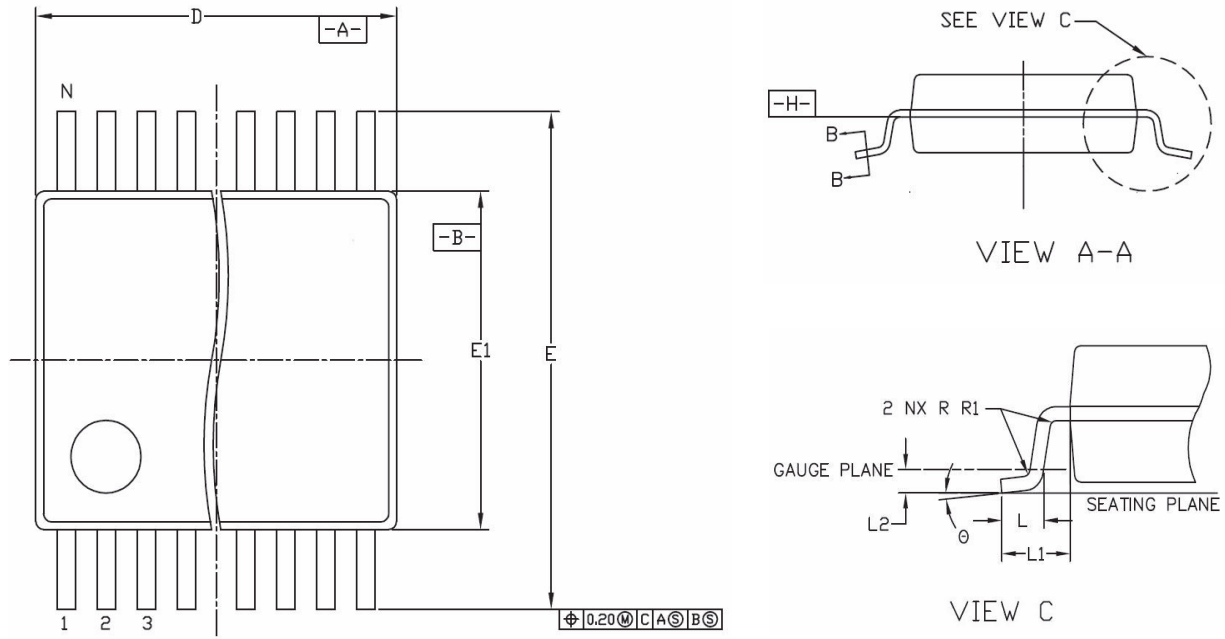
Figure 12. Package Drawings and Dimensions
