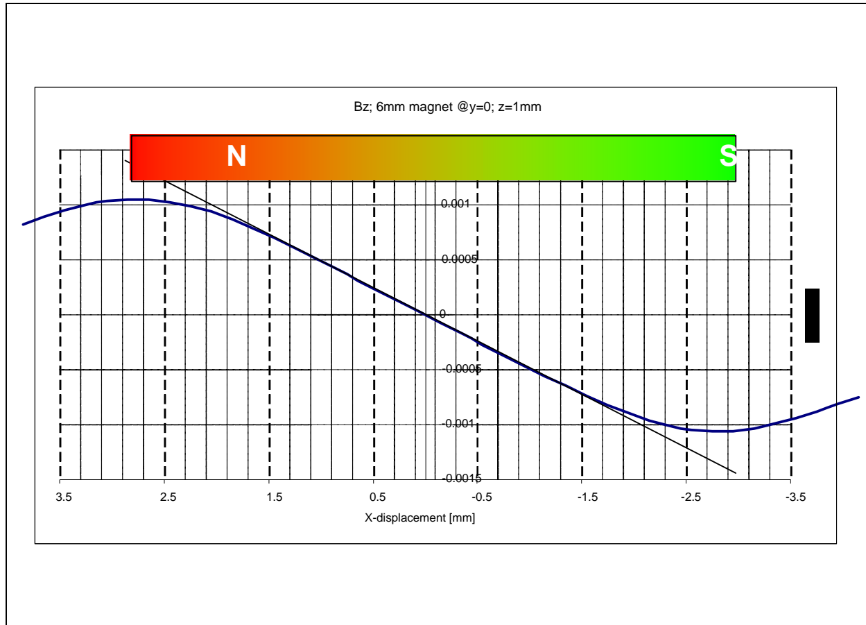
Figure 29. B_z Field Distribution Along the X-axis of a 6mm \varnothing Diametric Magnetized Magnet
