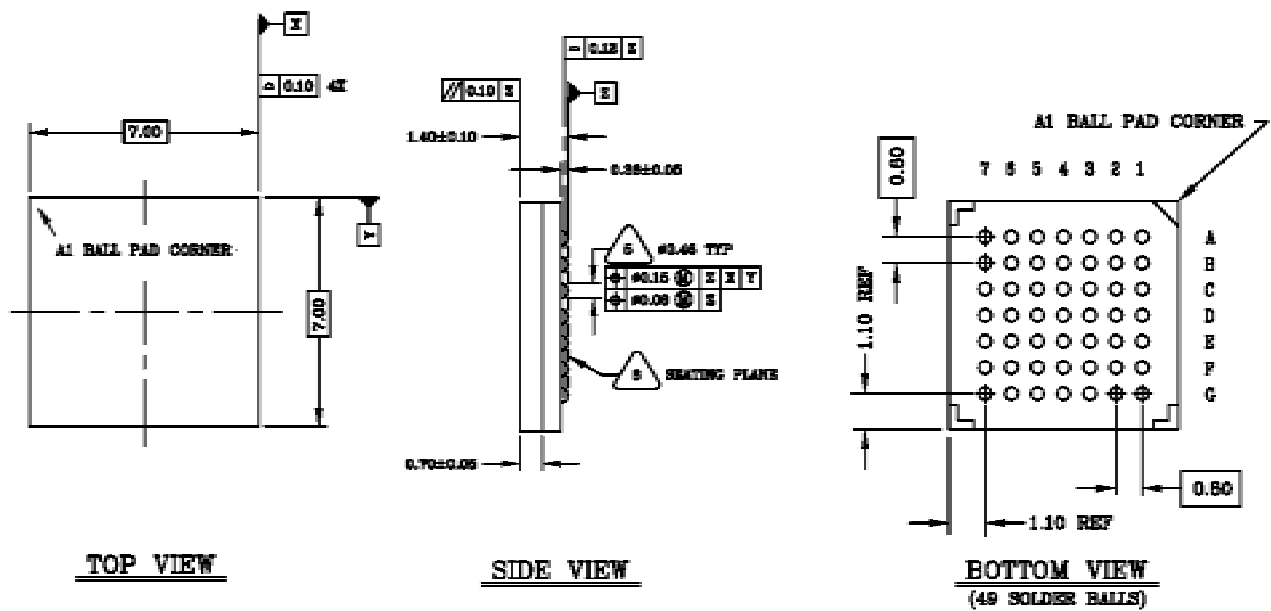
Figure 6 Mechanical Dimensions
