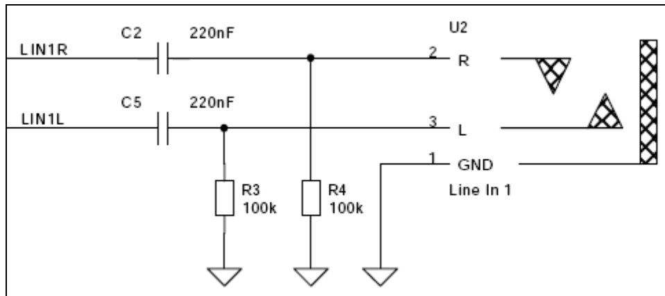
Figure 5 Line Input
