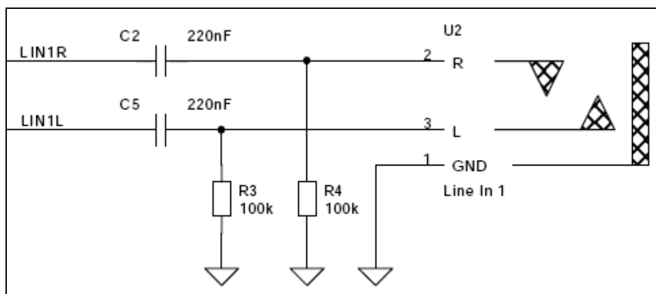
Figure 6 Line Input
