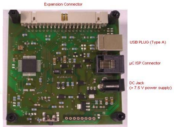
Figure 2: AS5130 demoboard, BOTTOM side
