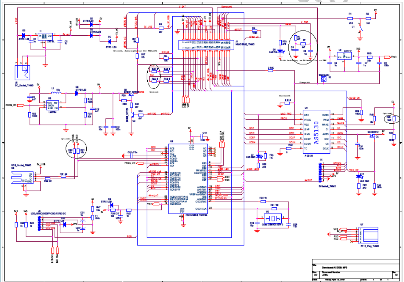
Figure 6: AS5130_DB_1.0 Demoboard schematics
