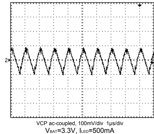
Figure 7 – Typical Operating Waveforms 1:1.5 Mode
