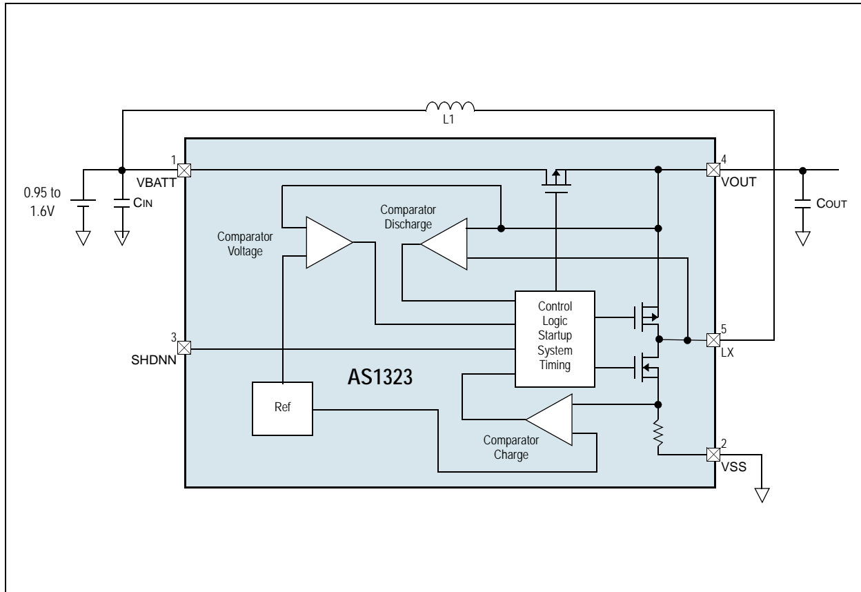
Figure 20. Block Diagram
