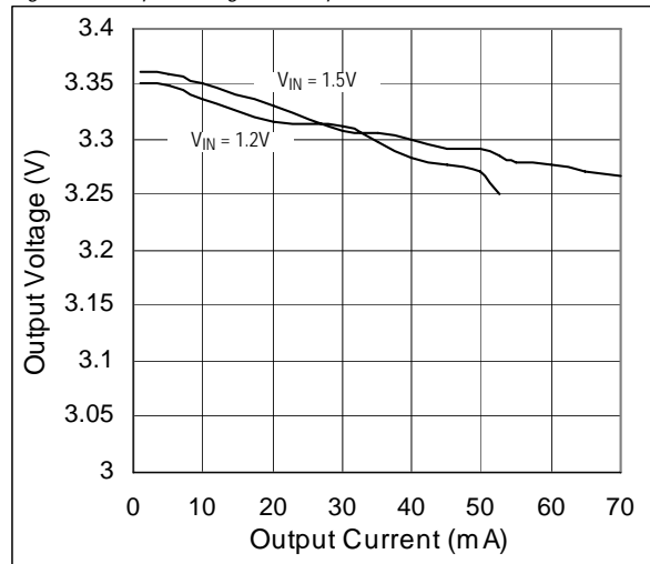
Figure 8. Output Voltage vs. Output Current
