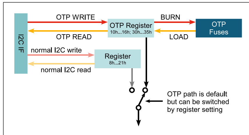
Figure 16. Register Access
