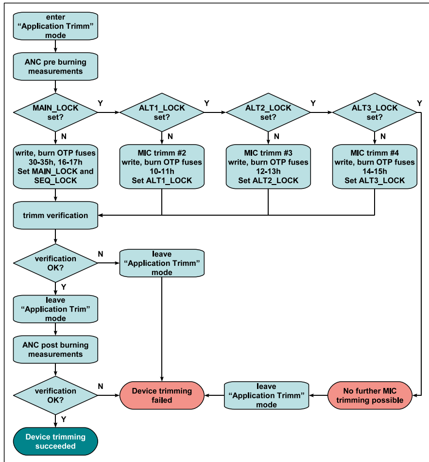
Figure 17. OTP Burning Process
