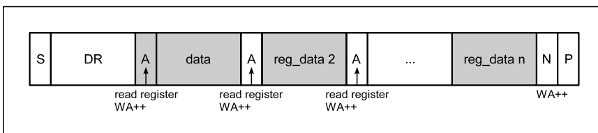
Figure 22. Current Address Read
