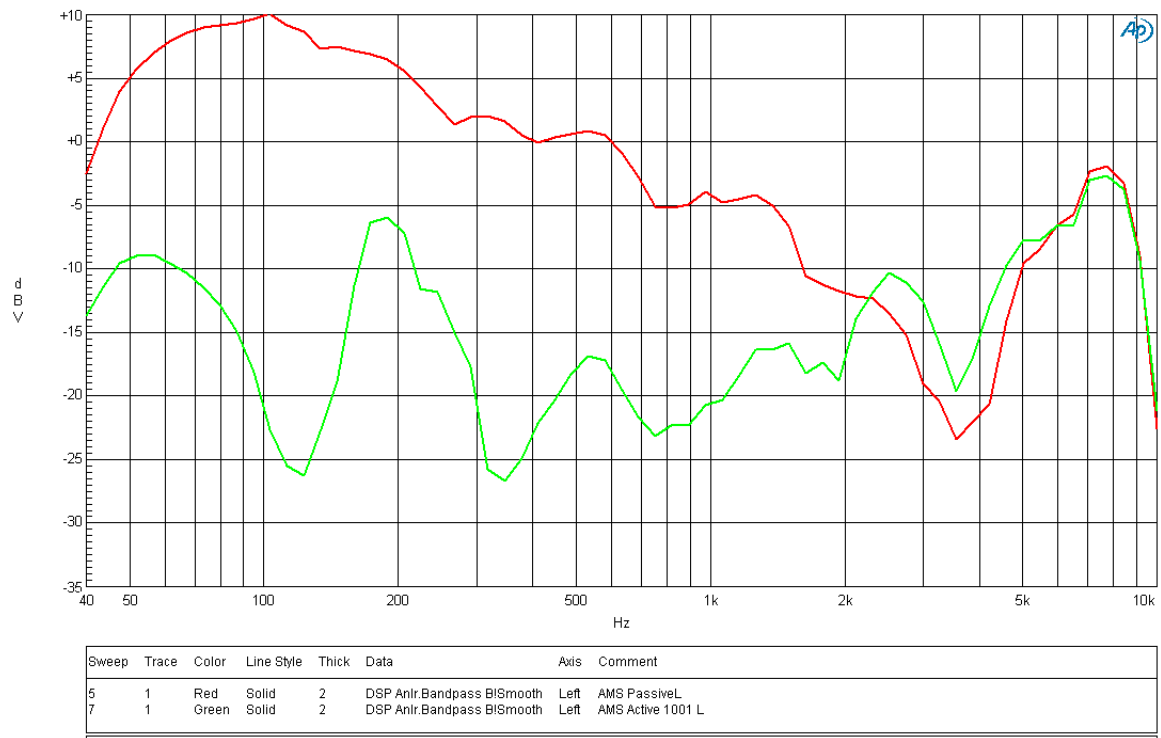
Figure 9. Typical Performance Data, FF configuration
