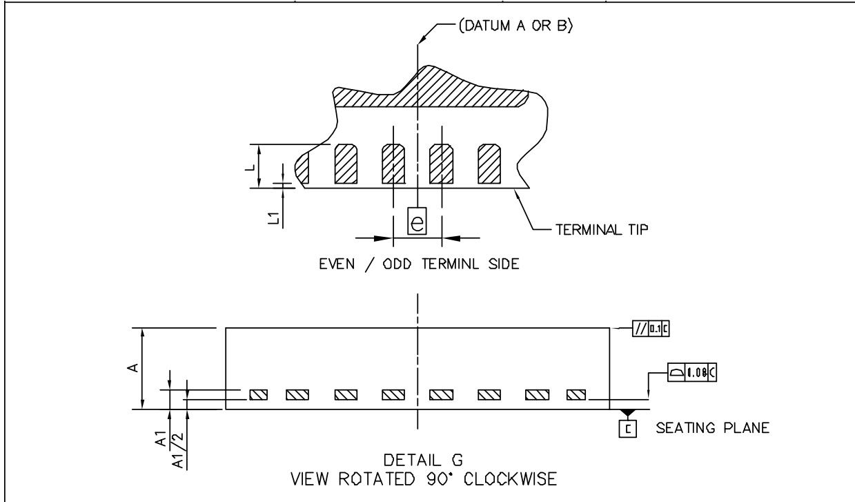
Figure 32. AS3400, AS3410; QFN24 0.5mm pitch details
