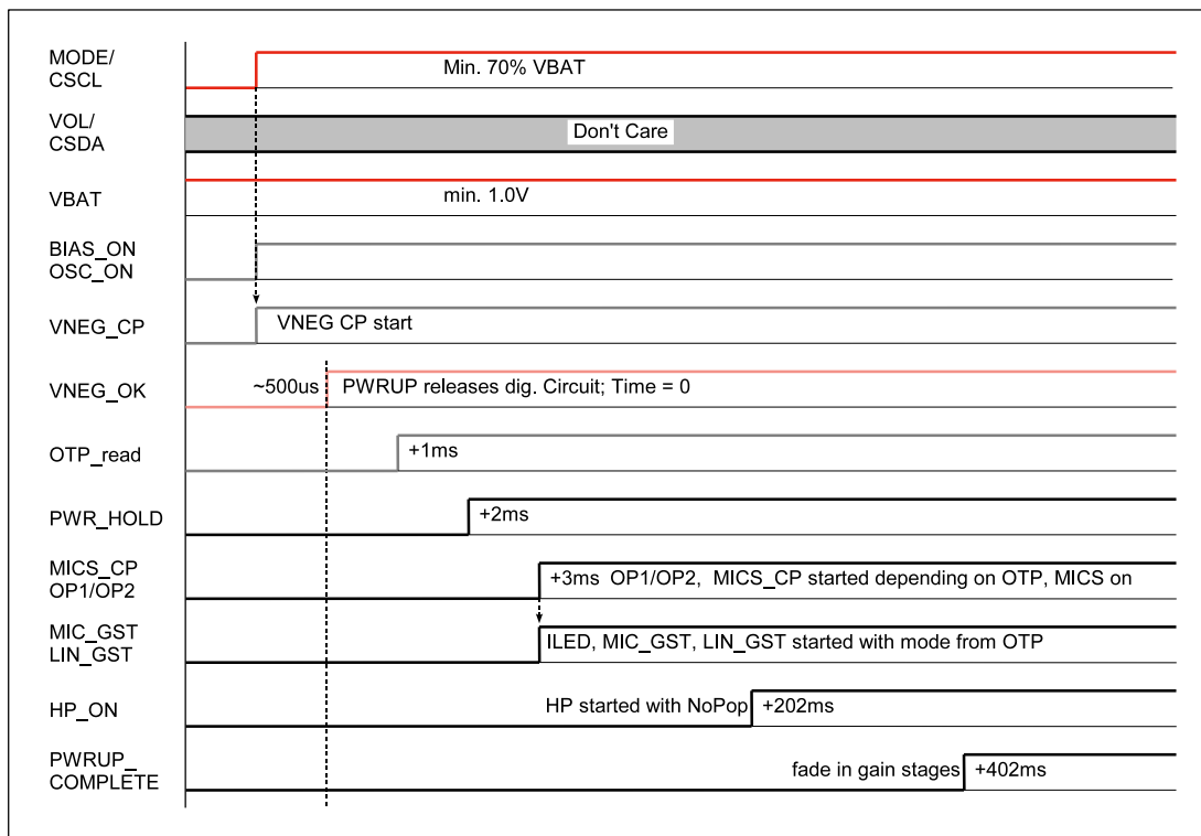
Figure 14. Stand-Alone Mode Start-Up Sequence
