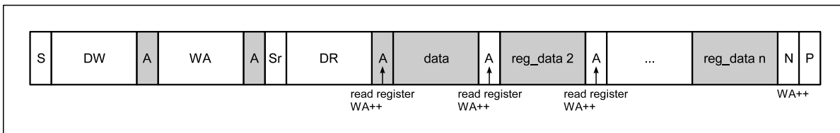
Figure 21. Sequential Read
