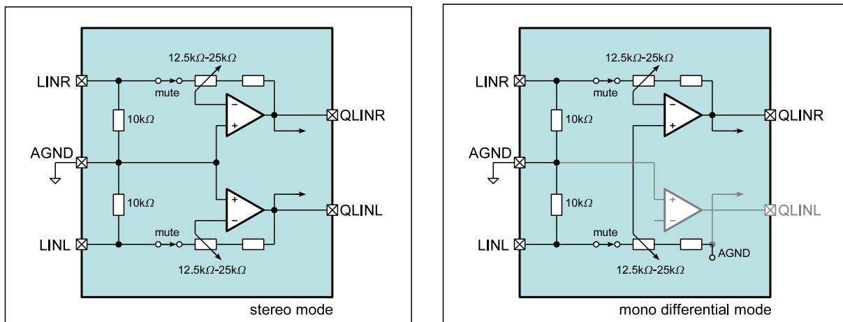
Figure 10. Line Inputs
