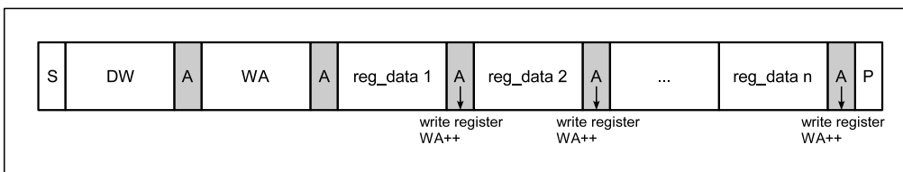
Figure 19. Page Write
