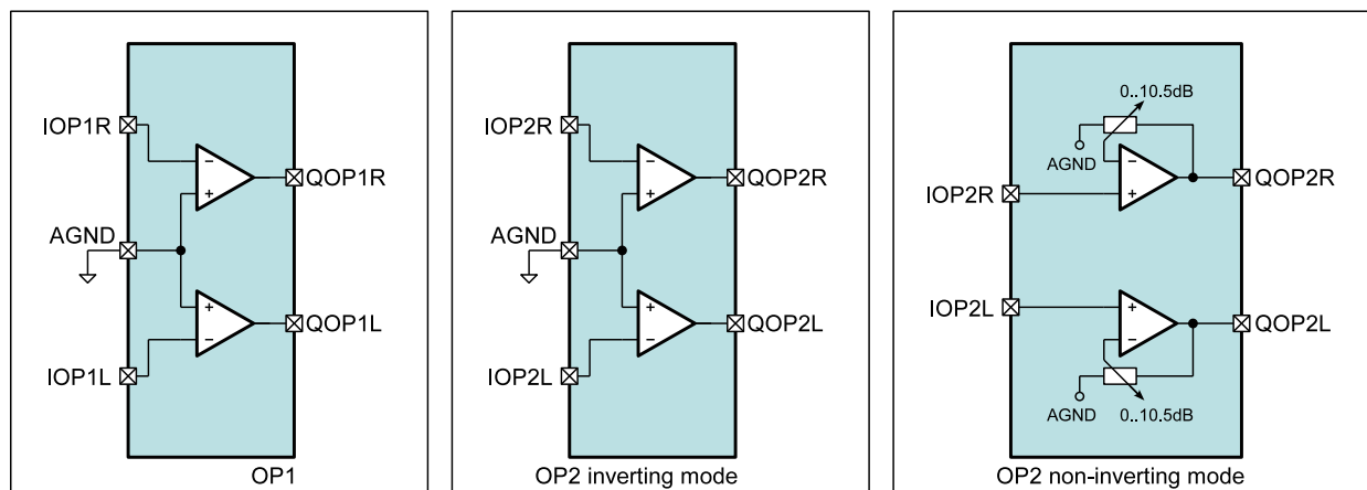
Figure 13. Operational Amplifiers
