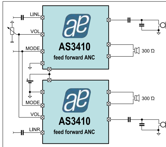
Figure 24. AS3410 High Performance Application in Bridged Mode for high impedance headsets
