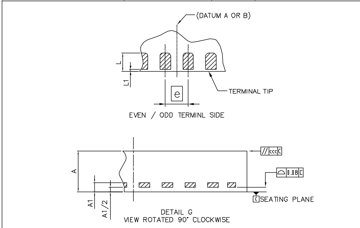
Figure 34. AS3430; QFN32 0.5mm pitch details
