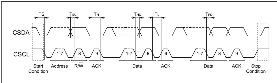
Figure 23. 2-Wire Serial Timing
