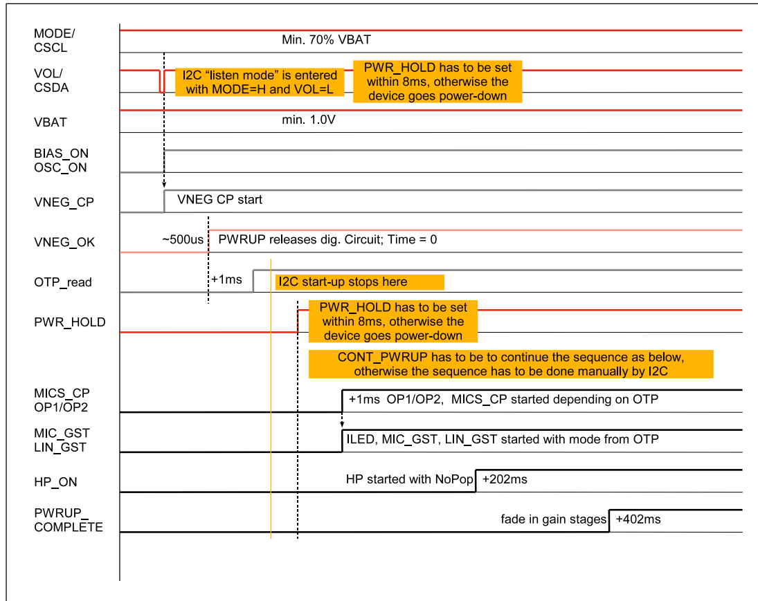
Figure 15. I2C Mode Start-Up Sequence
