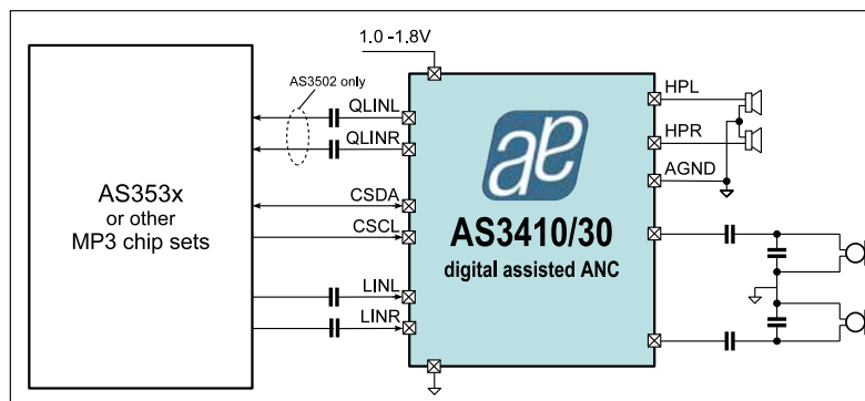
Figure 26. AS3430 on Music Player with ANC
