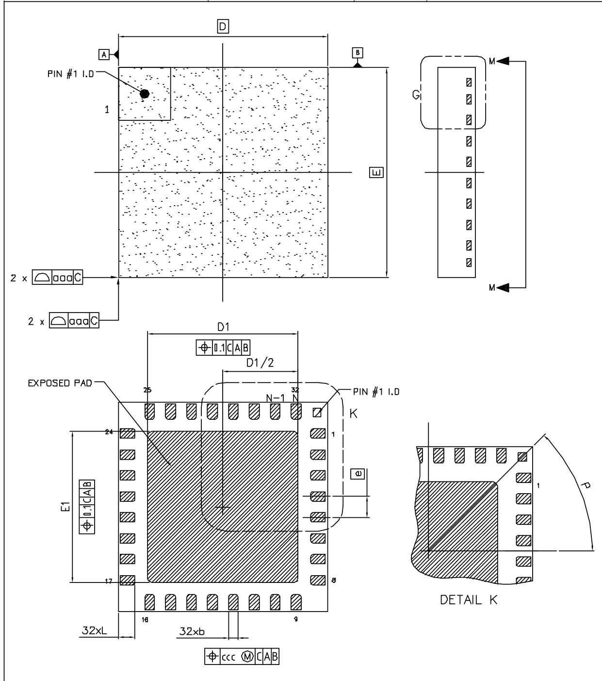
Figure 33. AS3430; QFN32 0.5mm pitch
