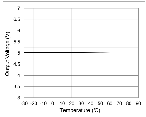
Figure 15. Buck - V_{OUT} vs. Temp.; V_{IN} = 24V
