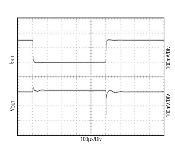
Figure 40. Load Transient; I_{OUT}=0mA to 150mA V_{IN}=2.0V , V_{OUT}=1.5V
