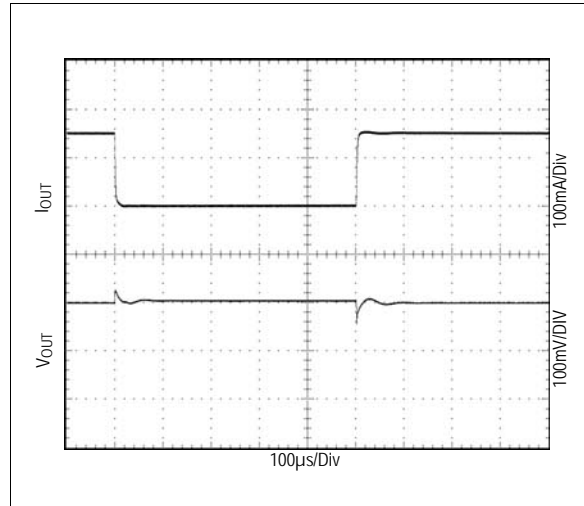
Figure 41. Load Transient; I_{OUT}=0mA to 150mA V_{IN}=3.3V , V_{OUT}=2.8V
